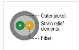
Uniboot Duplex Patch Cord cross section
