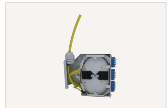
Splice box for top-hat rail mounting, open
