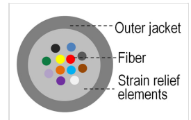
Fanout cable, cross section
