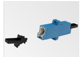
E-2000® (LSH) singlemode adapter
