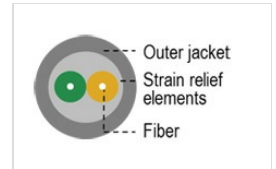
Duplex patch cable cross-section
