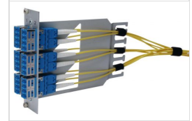
Fiber Optic Patch Module assembled
