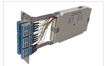
Compact Splice Module Twin LC
