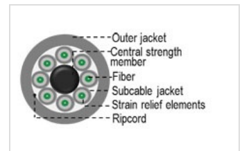
Breakout cable, cross section
