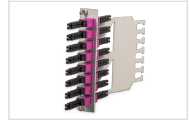
Base-8 patch module with MDC
